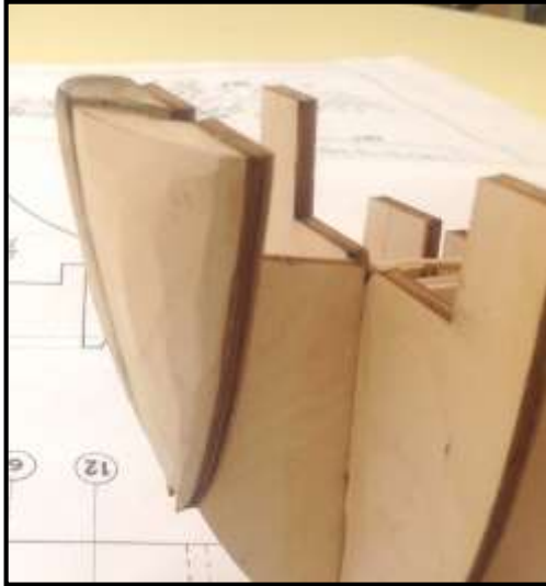
Figure 12: Preliminary Filler Block Shaping
